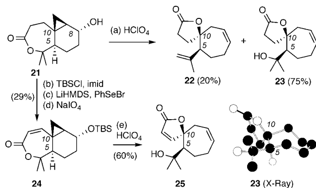
Scheme 3. Reagents and conditions: (a) 7% HClO 4 (1.0 equiv.), acetonitrile, H 2 O, 25 °C, 1.5 h, 75% of 23 and 20% of 22 ; (b) TBSCl (2.0 equiv.), imidazole (3.0 equiv.), DMAP (0.2 equiv.), DMF, 25 °C, 14 h, 92%; (c) LiHMDS (2.5 equiv.), PhSeBr (2.0 equiv.), THF, -78 °C, 1.5 h, 48%; (d) NaIO 4 (2.0 equiv.), THF/H 2 O (1:1), 0 °C, 2 h, 65%; (e) HClO 4 (1.0 equiv.), acetone, H 2 O, 25 °C, 2.0 h, 60%. LiHMDS: lithium bis(trimethylsilyl)amide, TBSCl: tert -butyldimethylsilyl chloride, DMAP: 4-(dimethylamino)-pyridine, DMF N,N -dimethylformamide.
